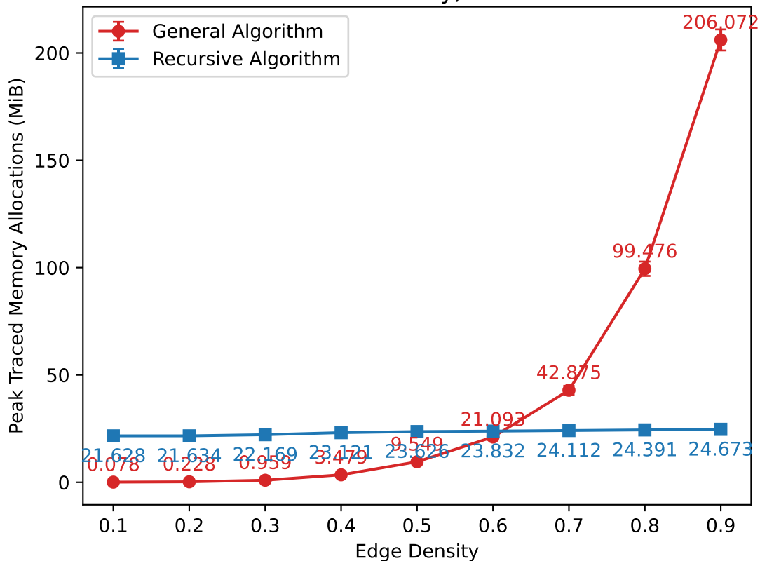
Peak Traced Allocations with Basis Tracking (10 isolated realizations per density)
